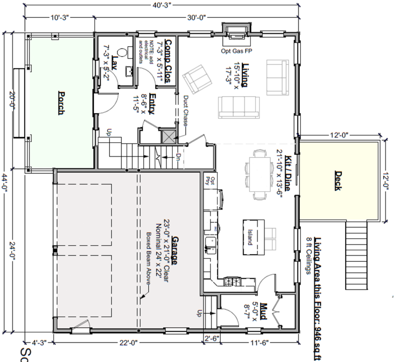
First Floor Plan Scale: 3/32" = 1'-0"
